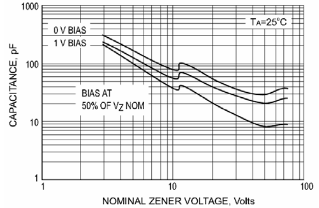
Fig.4 TYPICAL CAPACITANCE
