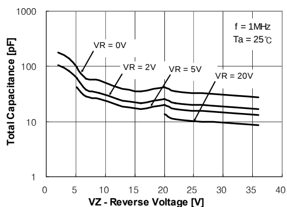
Figure 2. Total Capacitance
