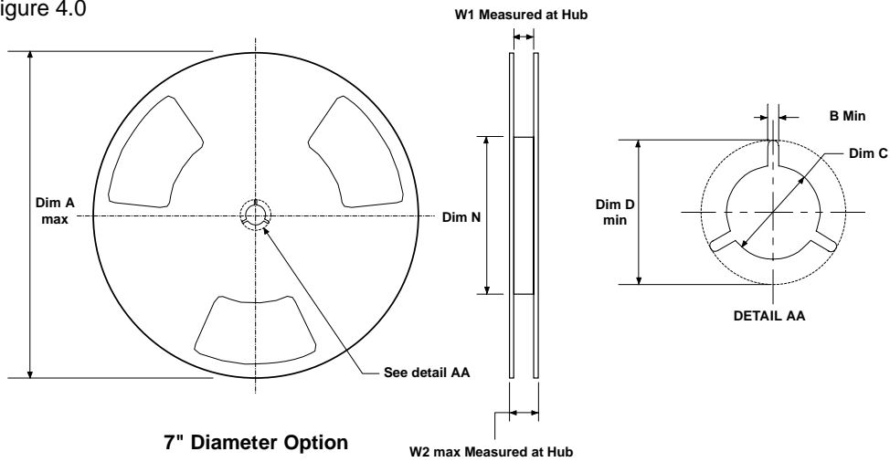
DO-214AC(SMA) Reel Configuration: Figure 4.0
